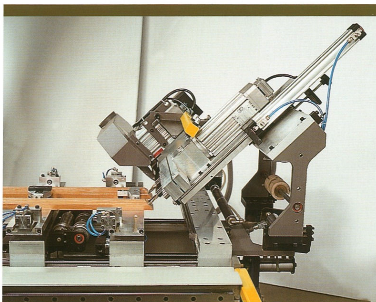
* Detalle grupo de taladro a 45 grados * Detail of the 45 degrees drilling group
